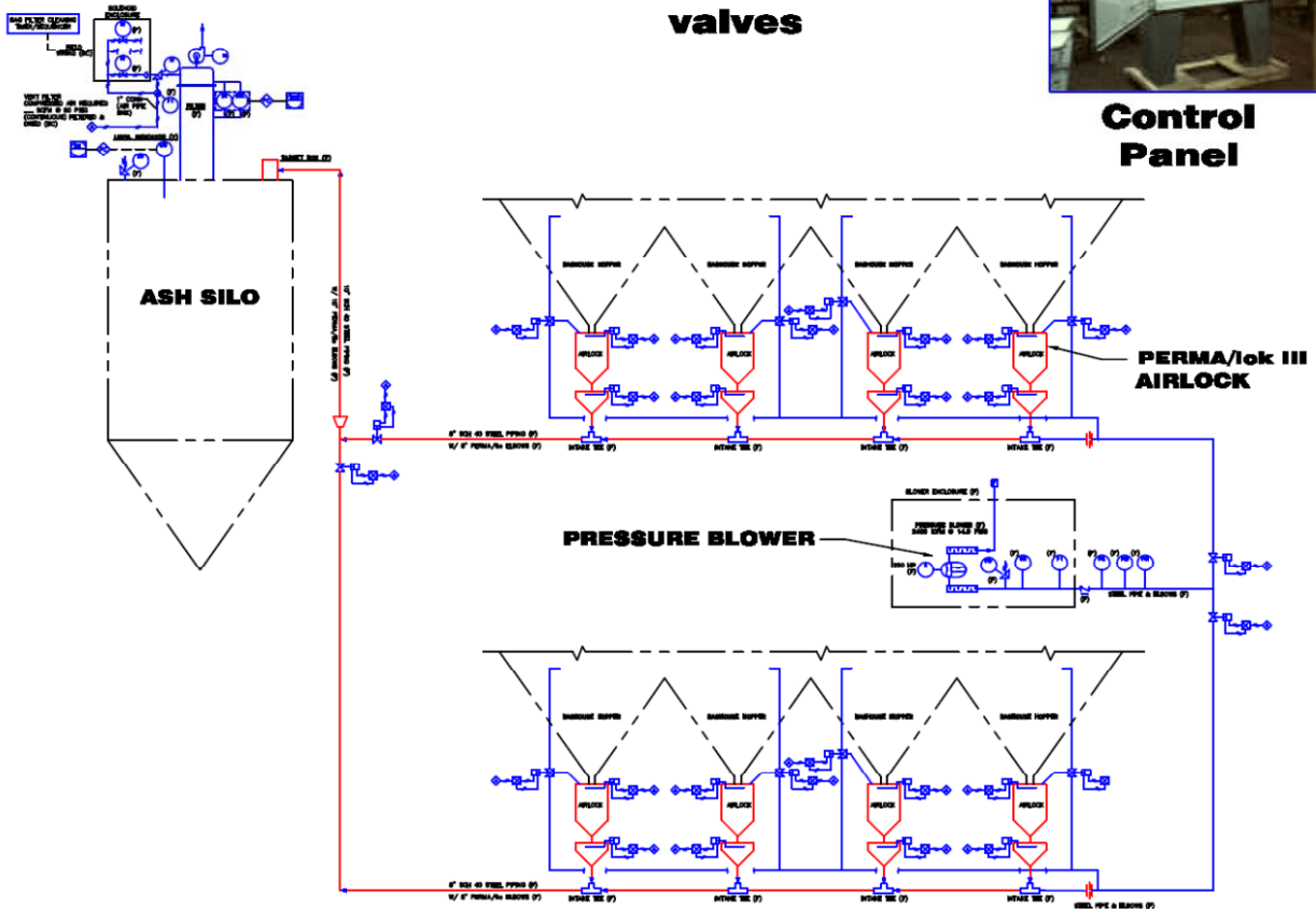
TYPICAL PRESSURE SYSTEM FLOW DIAGRAM
